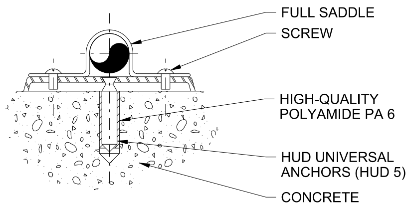
SECTIONAL VIEW
